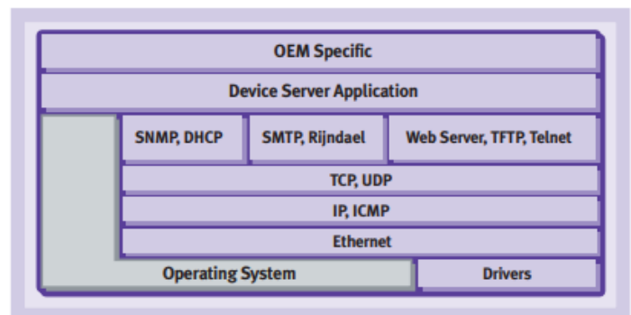
Internal Software Portfolio
