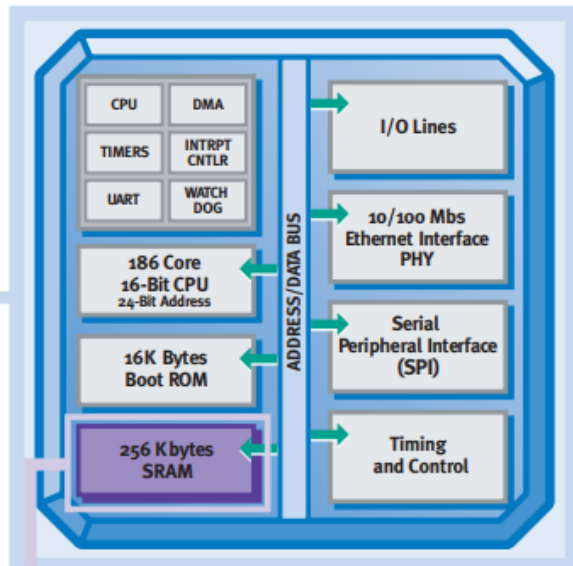
EX Chip Hardware Diagram
